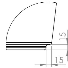
DETAIL 1 SCALE 1 : 5
